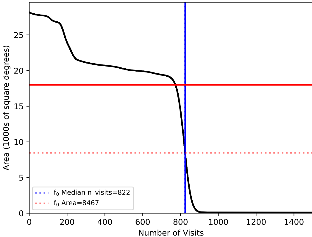
ddf_loaded_half_fl4_v3.4_10yrs All sky: fO
