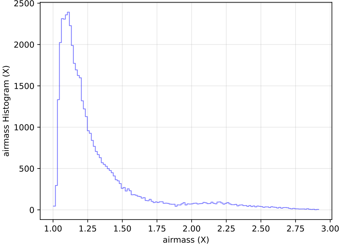
ddf_loaded_half_fl4_v3.4_10yrs Yr 1 z band: airmass Histogram
