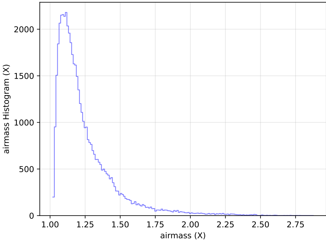
ddf_loaded_half_fl4_v3.4_10yrs Yr 1 y band: airmass Histogram
