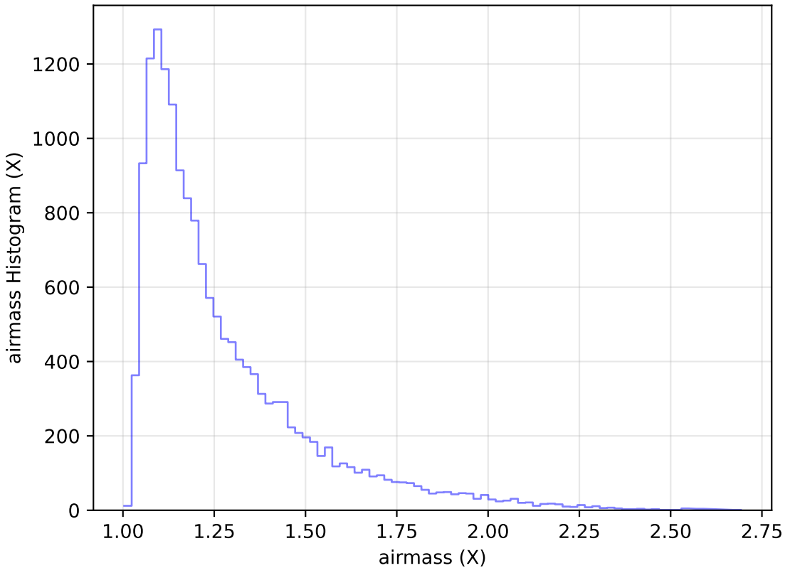
ddf_loaded_half_fl4_v3.4_10yrs Yr 1 u band: airmass Histogram
