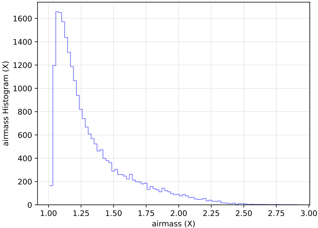
ddf_loaded_half_fl4_v3.4_10yrs Yr 1 g band: airmass Histogram
