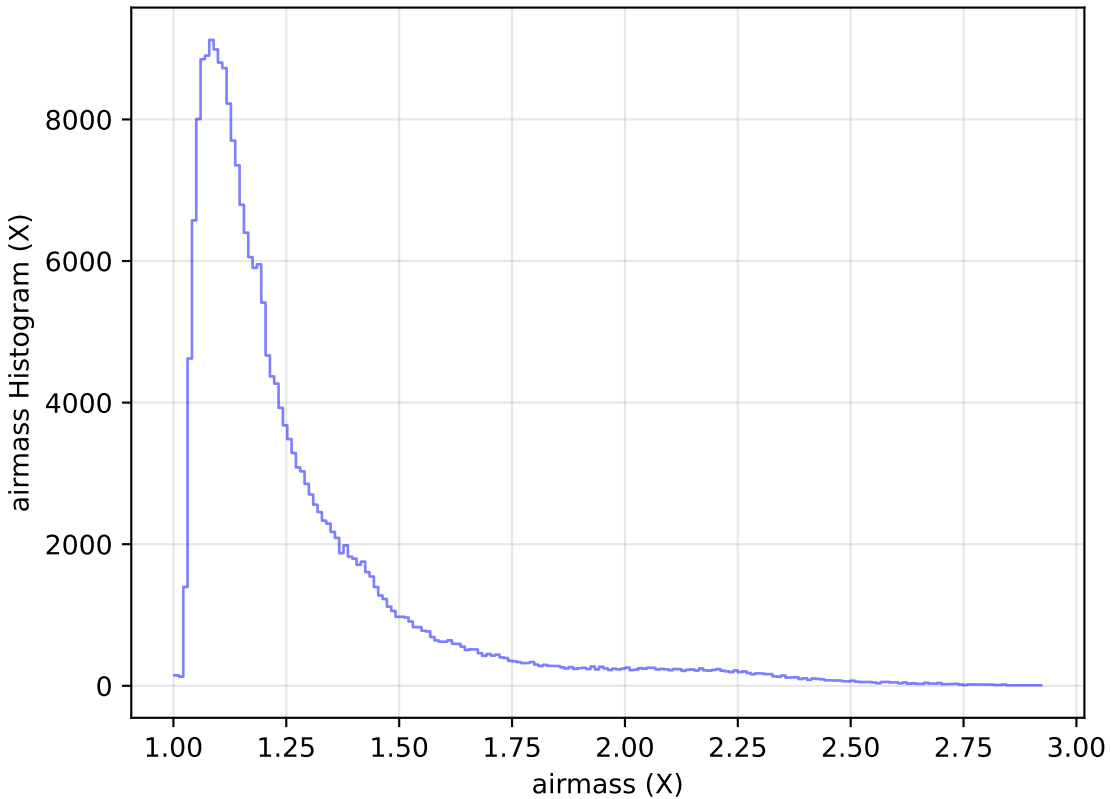
ddf_loaded_half_fl4_v3.4_10yrs Yr 1 all bands: airmass Histogram
