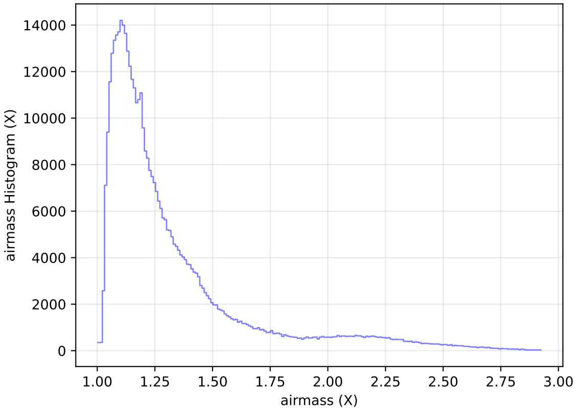
ddf_loaded_half_fl4_v3.4_10yrs WFD z band: airmass Histogram
