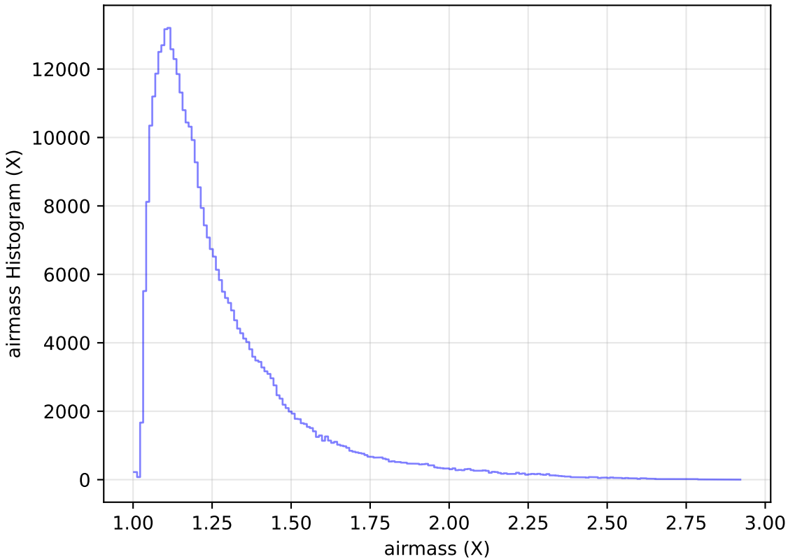
ddf_loaded_half_fl4_v3.4_10yrs WFD y band: airmass Histogram
