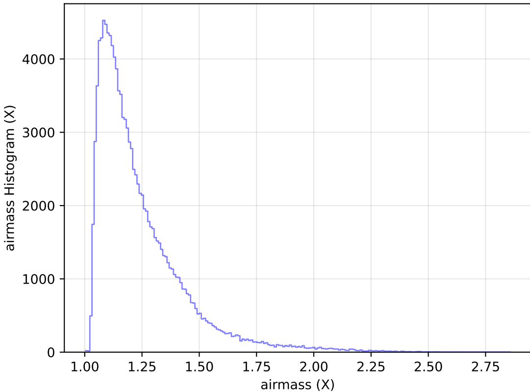
ddf_loaded_half_fl4_v3.4_10yrs WFD u band: airmass Histogram
