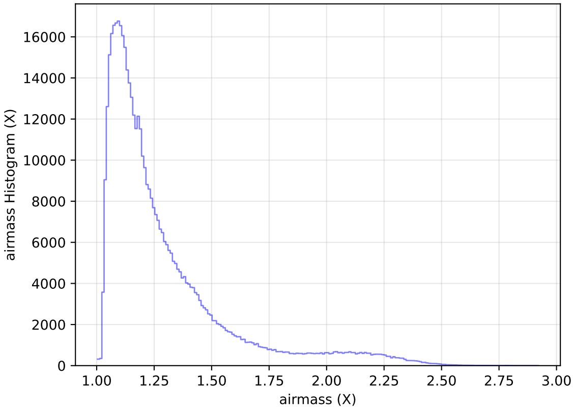
ddf_loaded_half_fl4_v3.4_10yrs WFD r band: airmass Histogram
