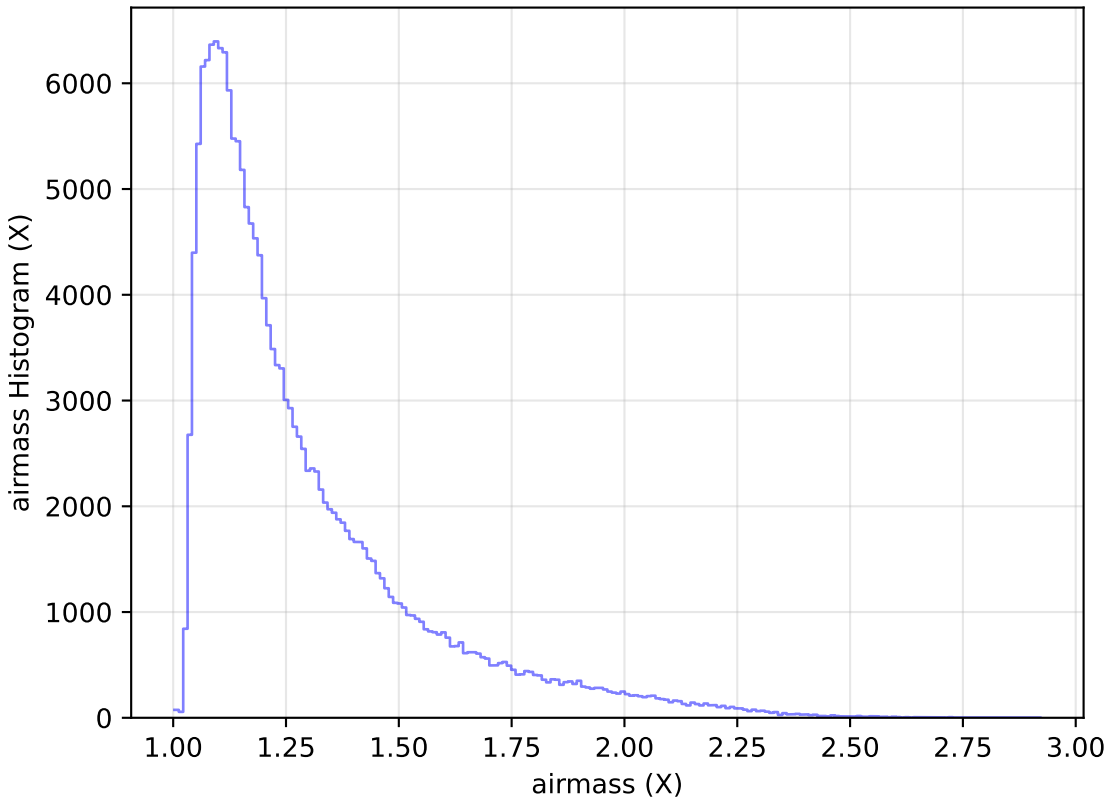
ddf_loaded_half_fl4_v3.4_10yrs WFD g band: airmass Histogram
