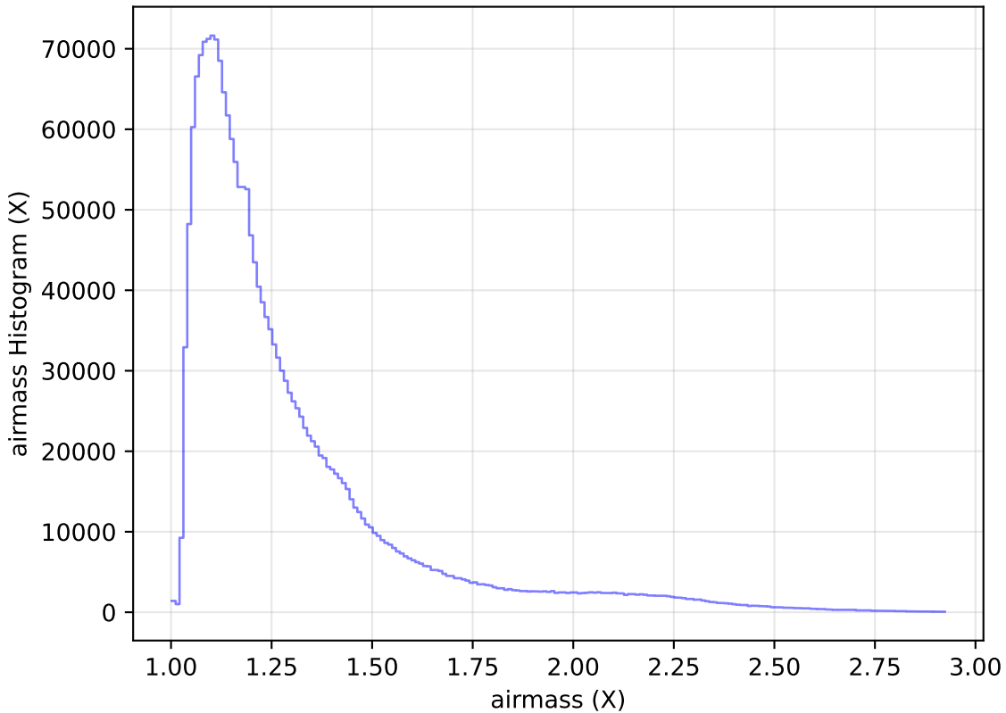
ddf_loaded_half_fl4_v3.4_10yrs WFD all bands: airmass Histogram
