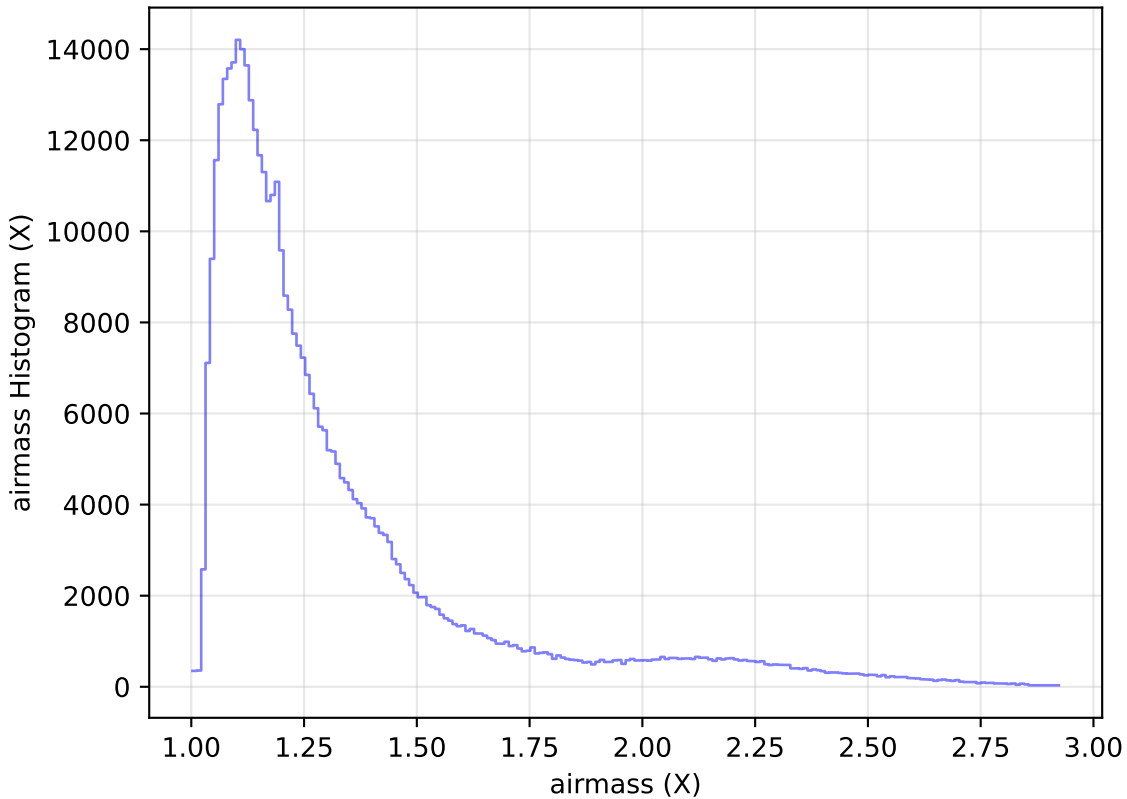
ddf_loaded_half_fl4_v3.4_10yrs All sky z band: airmass Histogram
