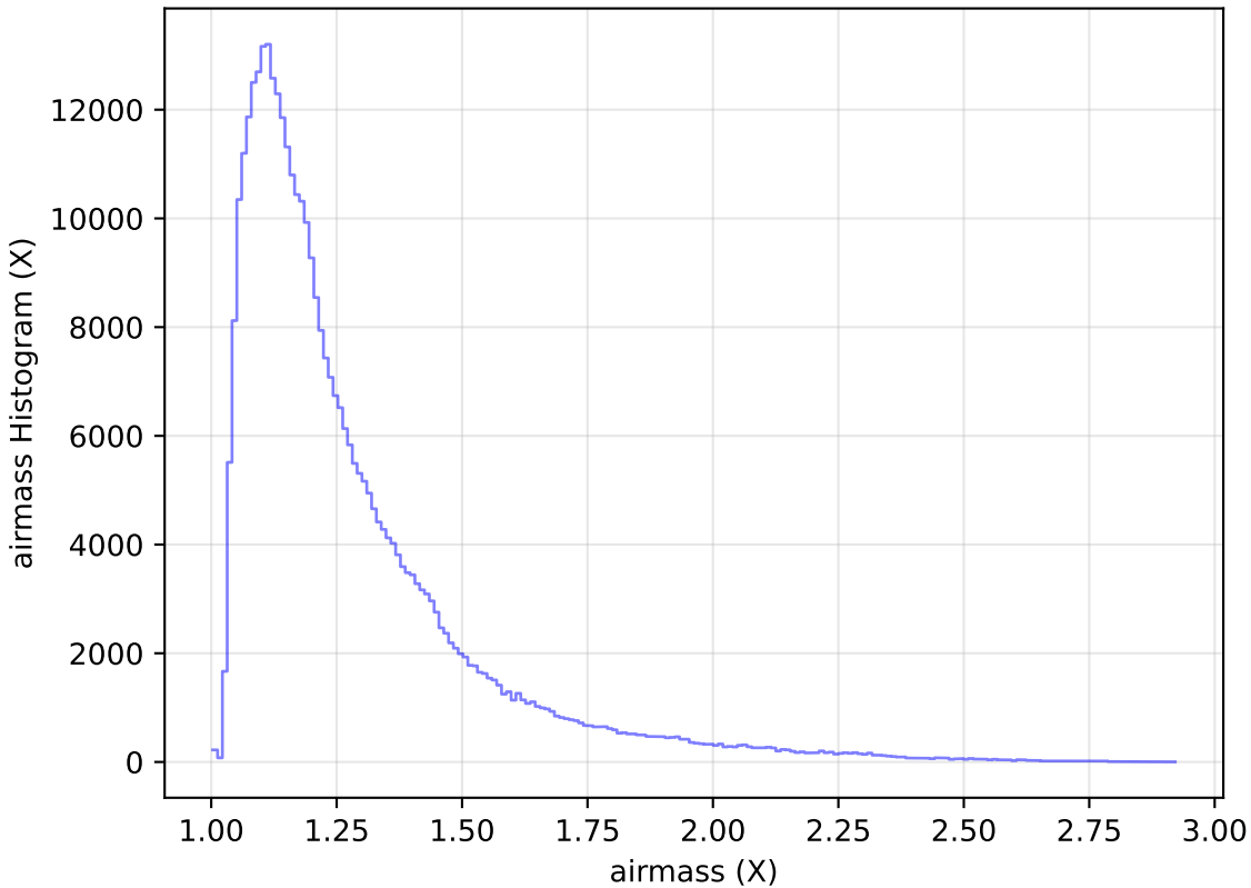
ddf_loaded_half_fl4_v3.4_10yrs All sky y band: airmass Histogram
