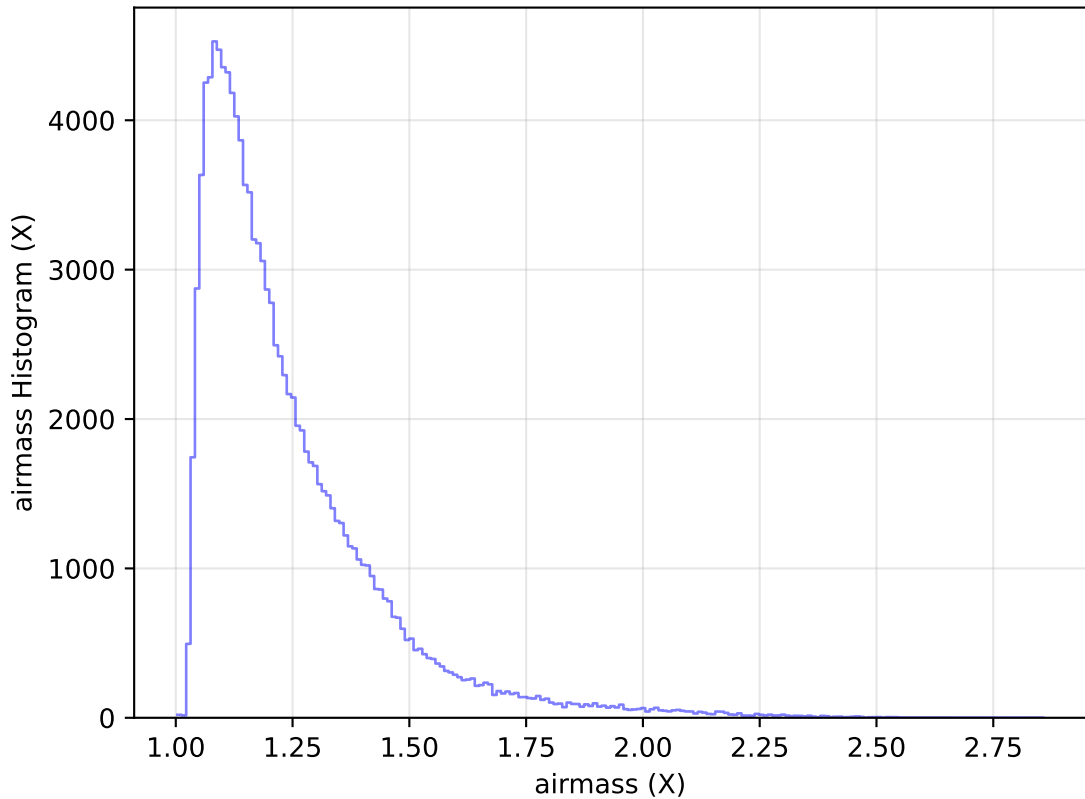
ddf_loaded_half_fl4_v3.4_10yrs All sky u band: airmass Histogram
