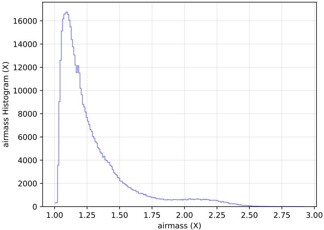
ddf_loaded_half_fl4_v3.4_10yrs All sky r band: airmass Histogram
