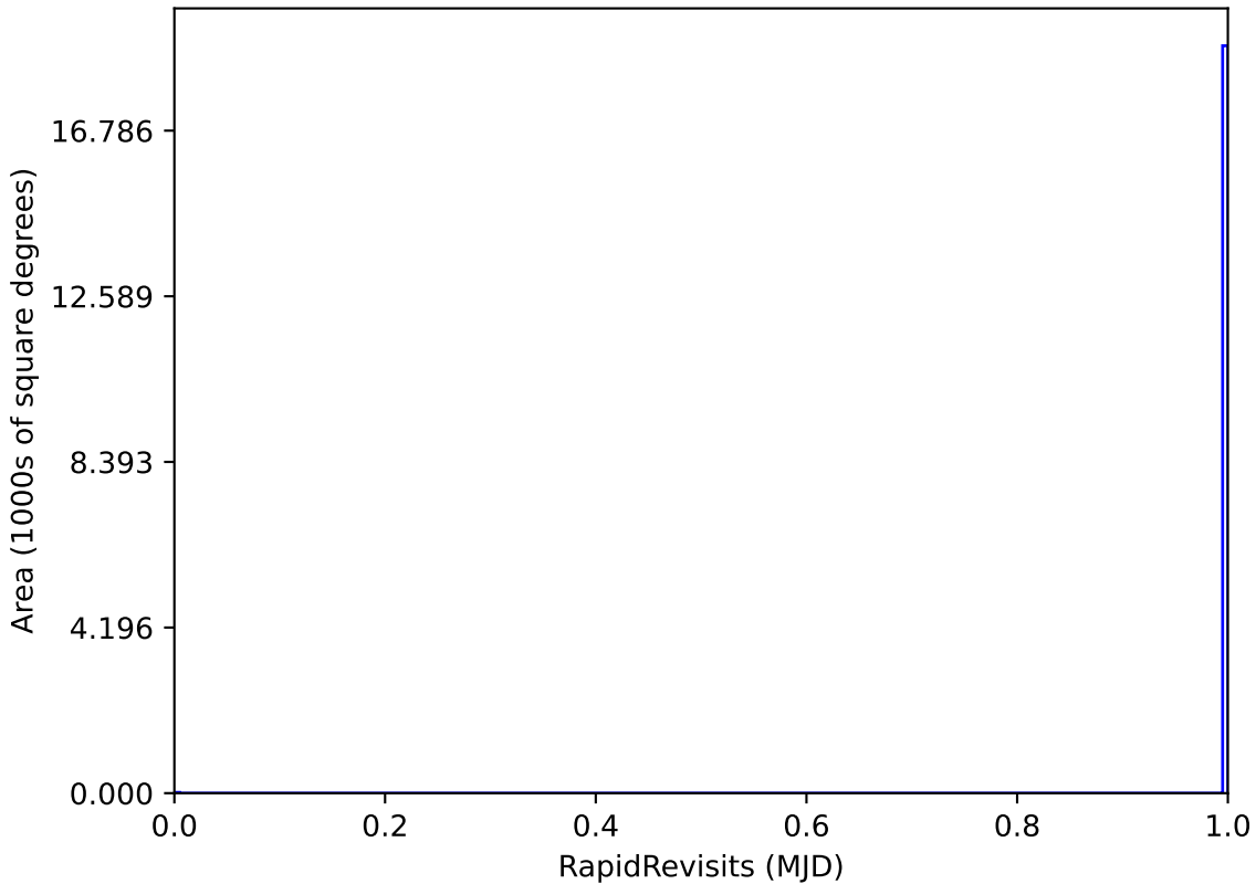
ddf_loaded_half_fl4_v3.4_10yrs WFD: RapidRevisits
