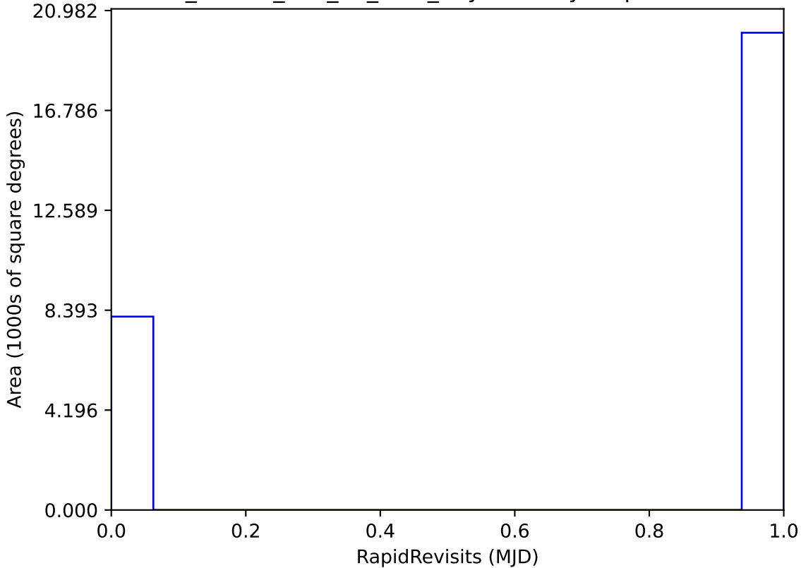
ddf_loaded_half_fl4_v3.4_10yrs All sky: RapidRevisits
