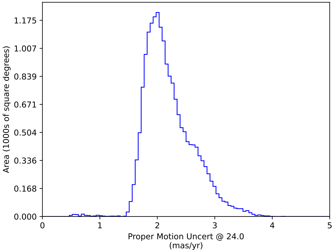
ddf_loaded_half_fl4_v3.4_10yrs WFD: Proper Motion Uncert @ 24.0
