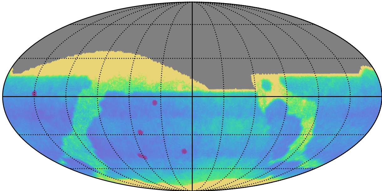
ddf_loaded_half_fl4_v3.4_10yrs All sky: Proper Motion Uncert @ 24.0
