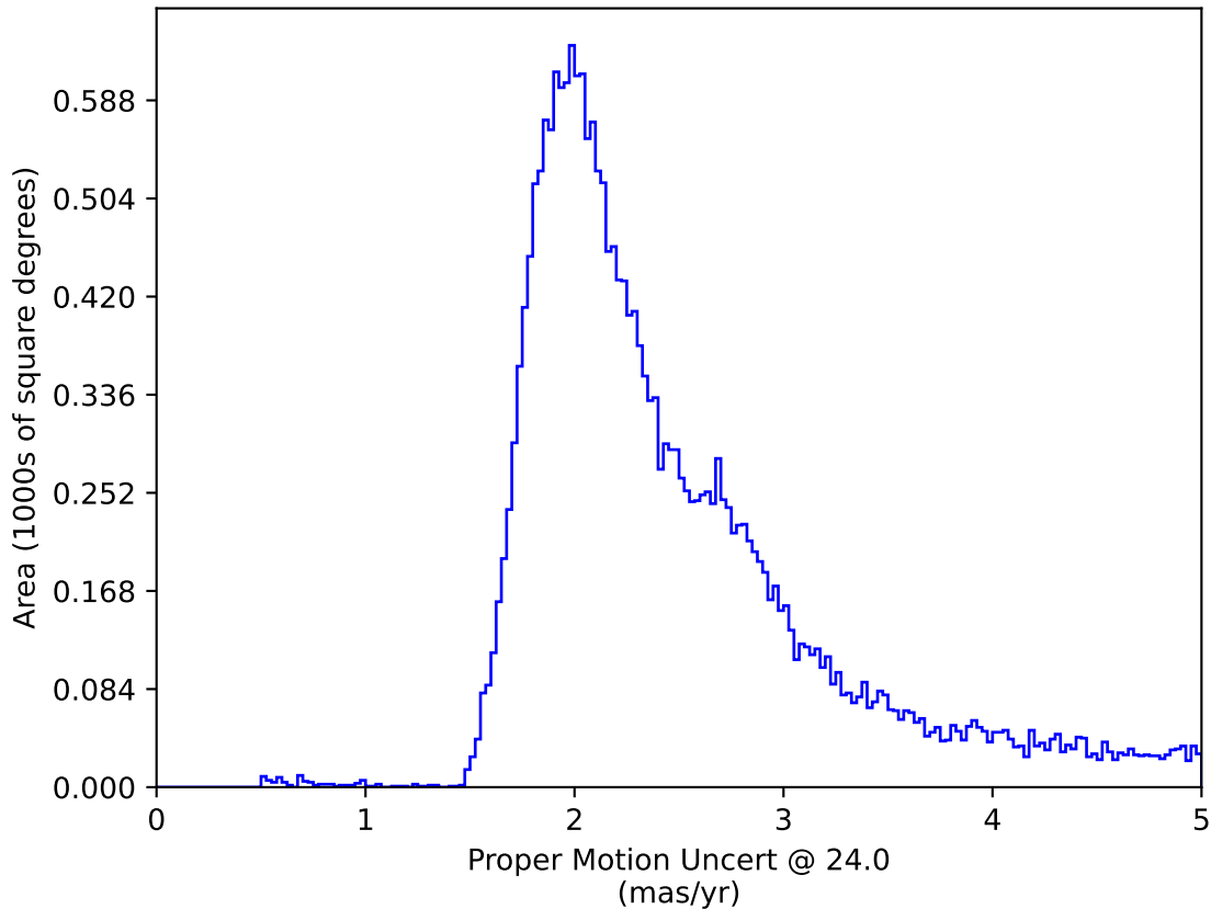
ddf_loaded_half_fl4_v3.4_10yrs All sky: Proper Motion Uncert @ 24.0
