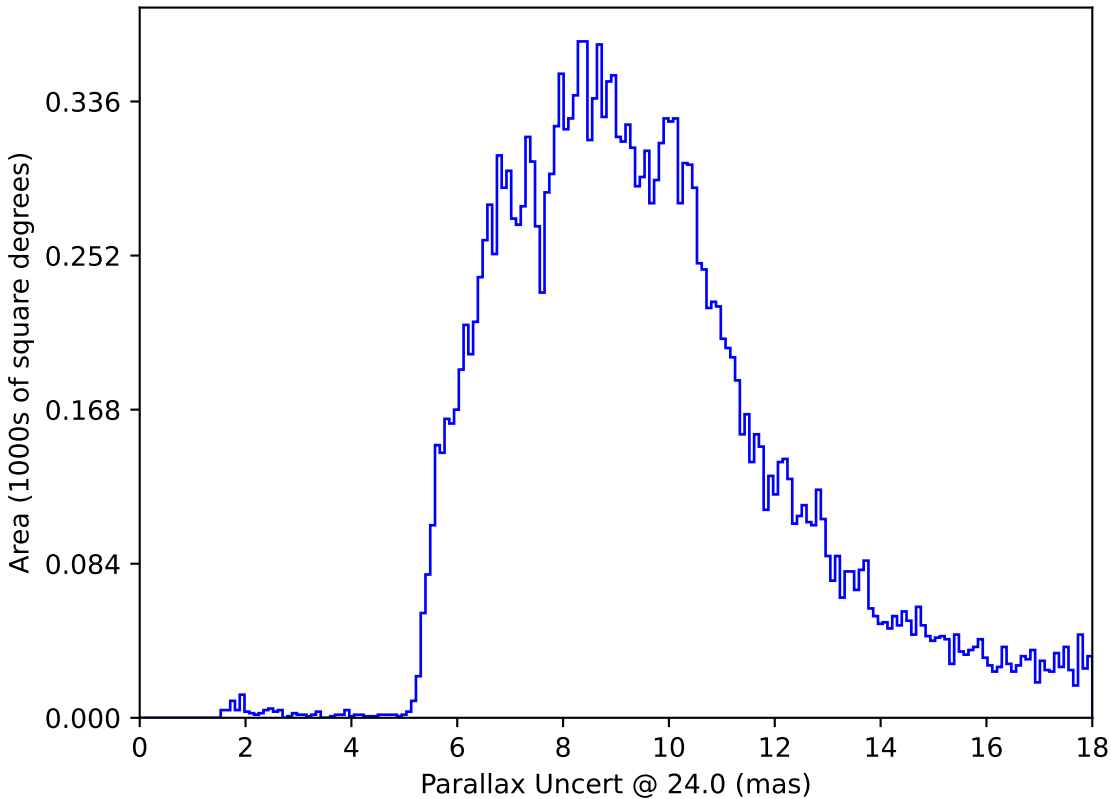
ddf_loaded_half_fl4_v3.4_10yrs All sky: Parallax Uncert @ 24.0
