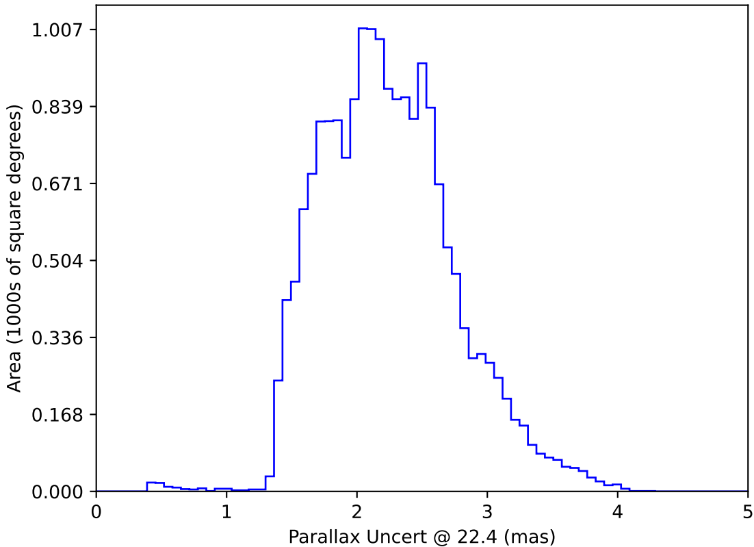
ddf_loaded_half_fl4_v3.4_10yrs WFD: Parallax Uncert @ 22.4
