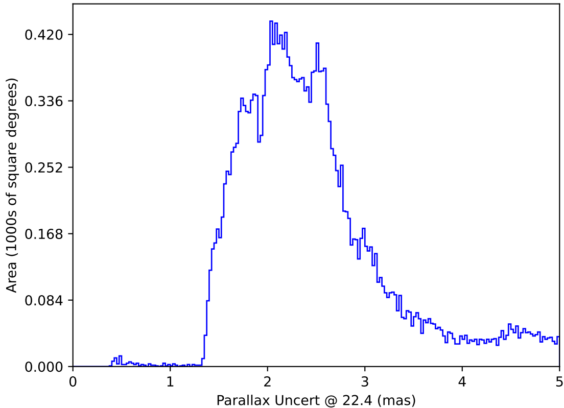
ddf_loaded_half_fl4_v3.4_10yrs All sky: Parallax Uncert @ 22.4
