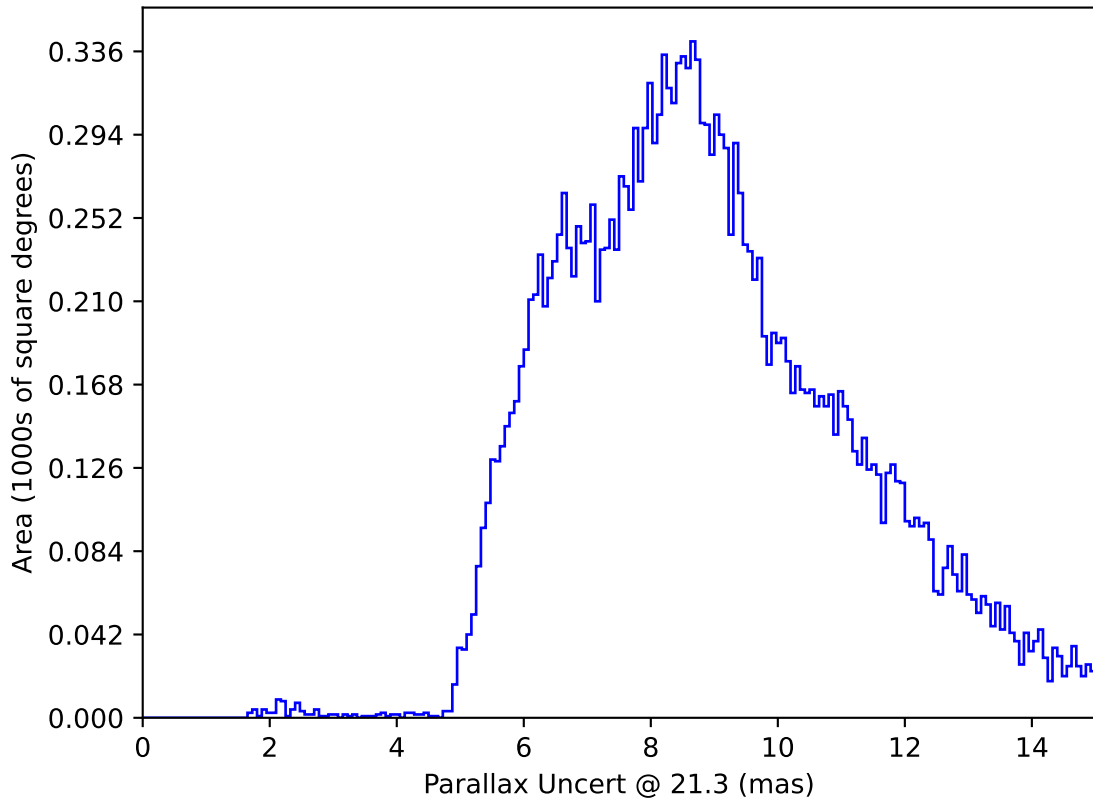
ddf_loaded_half_fl4_v3.4_10yrs All sky y band only: Parallax Uncert @ 21.3
