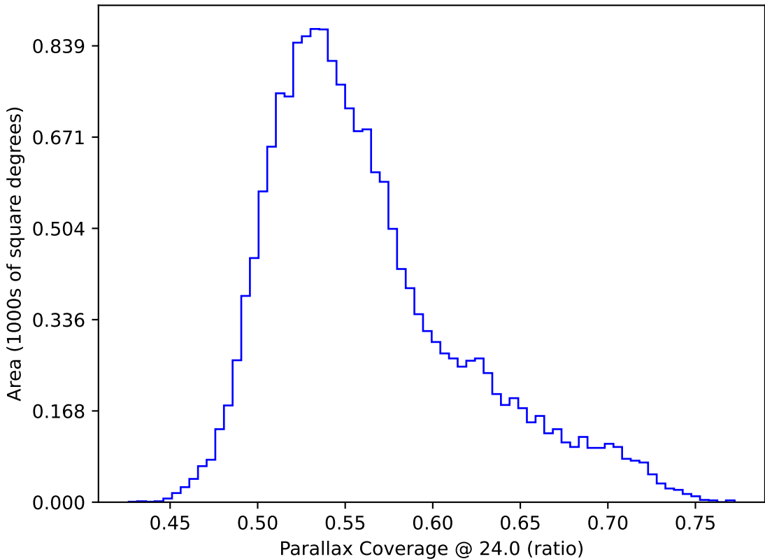
ddf_loaded_half_fl4_v3.4_10yrs WFD: Parallax Coverage @ 24.0
