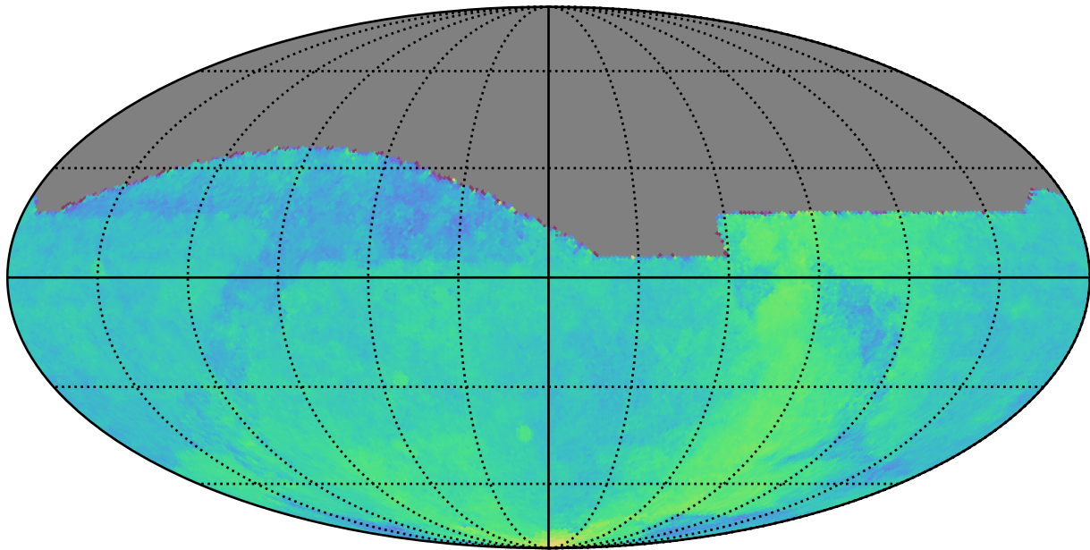
ddf_loaded_half_fl4_v3.4_10yrs All sky: Parallax Coverage @ 24.0
