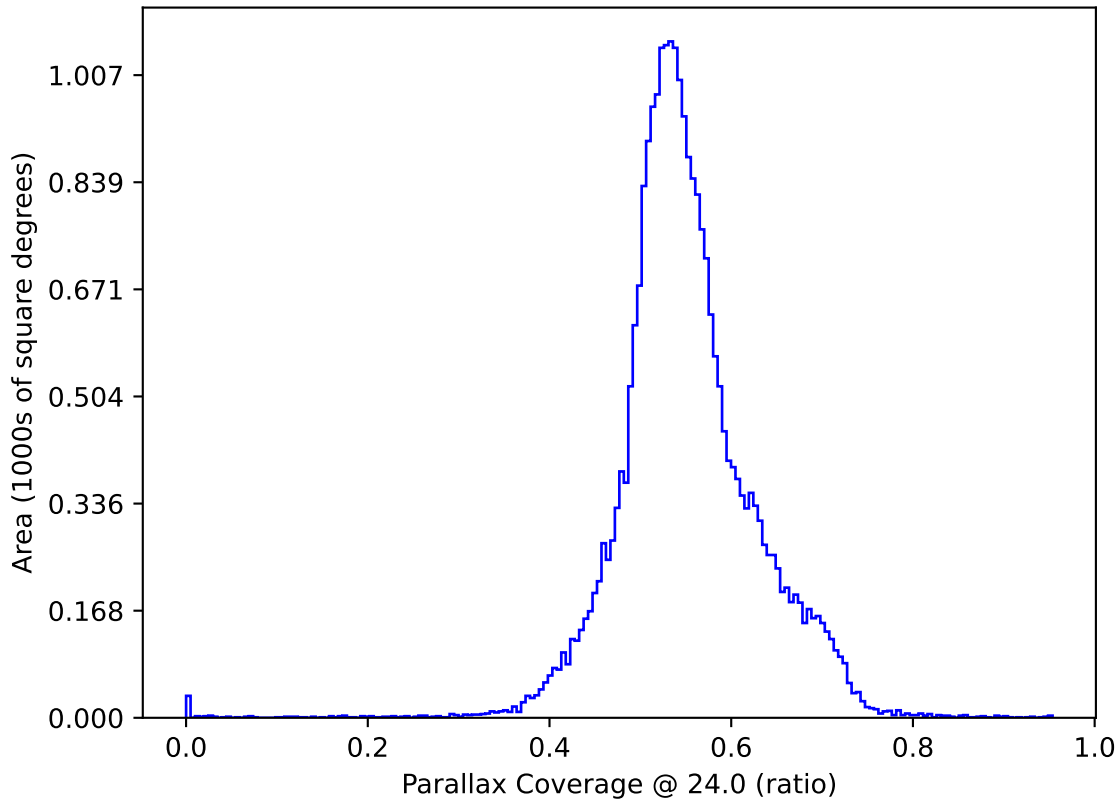
ddf_loaded_half_fl4_v3.4_10yrs All sky: Parallax Coverage @ 24.0
