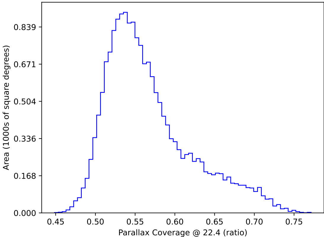
ddf_loaded_half_fl4_v3.4_10yrs WFD: Parallax Coverage @ 22.4
