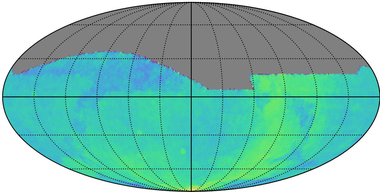
ddf_loaded_half_fl4_v3.4_10yrs All sky: Parallax Coverage @ 22.4
