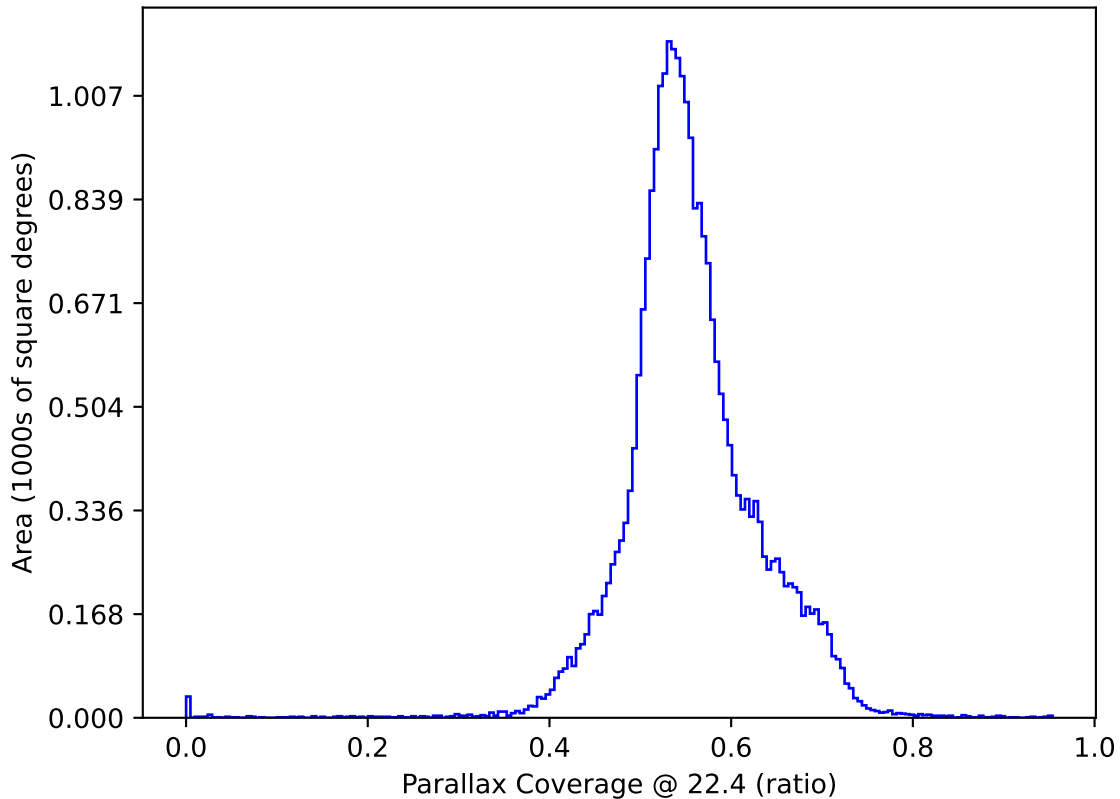
ddf_loaded_half_fl4_v3.4_10yrs All sky: Parallax Coverage @ 22.4
