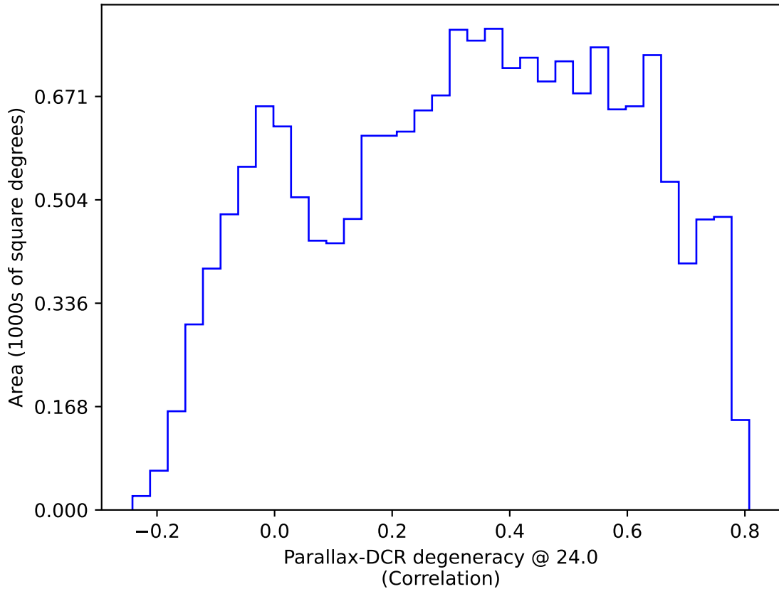
ddf_loaded_half_fl4_v3.4_10yrs WFD: Parallax-DCR degeneracy @ 24.0
