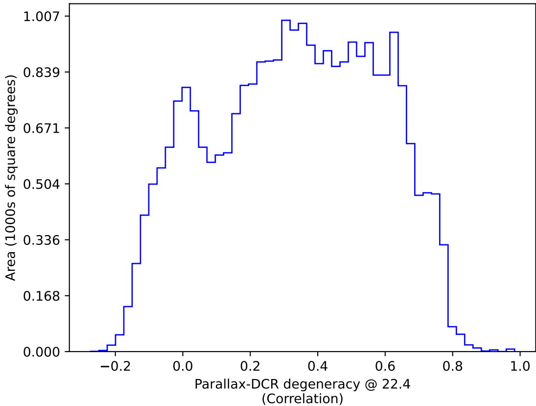
ddf_loaded_half_fl4_v3.4_10yrs All sky: Parallax-DCR degeneracy @ 22.4
