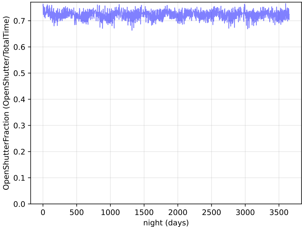
ddf_loaded_half_fl4_v3.4_10yrs Per night: OpenShutterFraction
