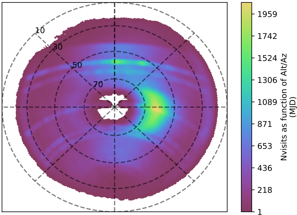
ddf_loaded_half_fl4_v3.4_10yrs z band: Nvisits as function of Alt/Az
