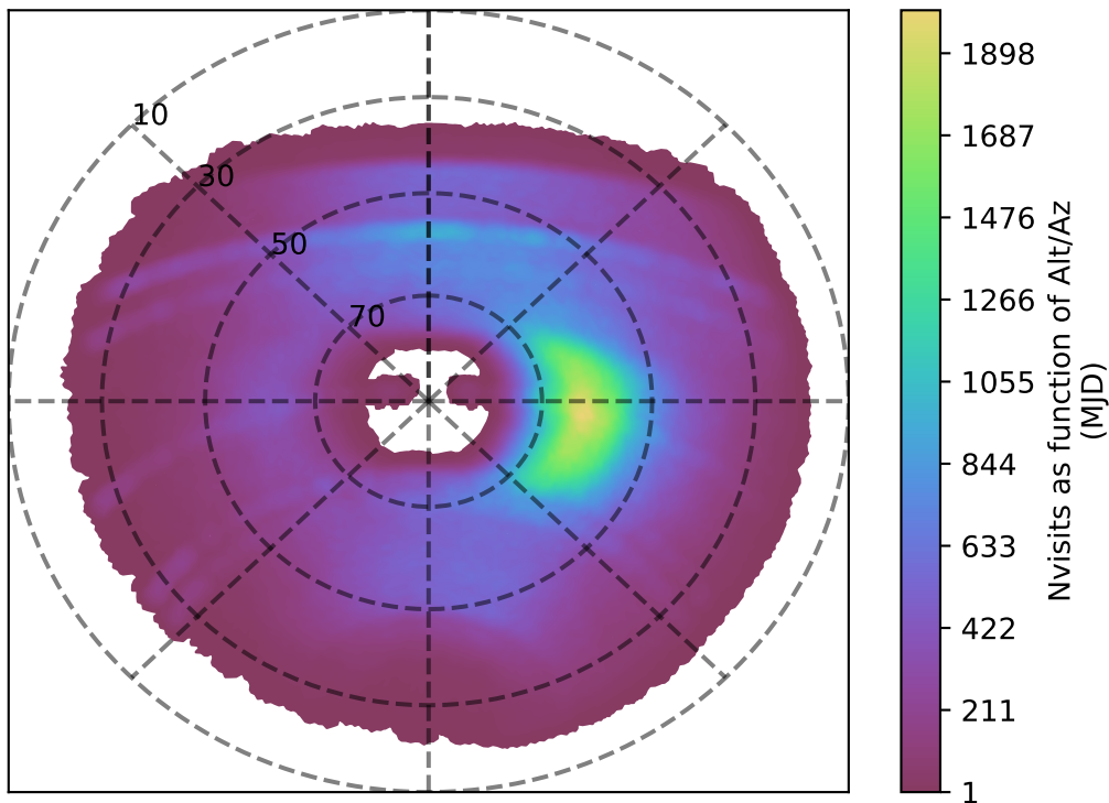
ddf_loaded_half_fl4_v3.4_10yrs y band: Nvisits as function of Alt/Az
