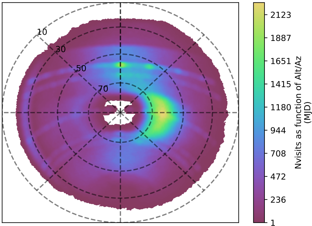
ddf_loaded_half_fl4_v3.4_10yrs r band: Nvisits as function of Alt/Az
