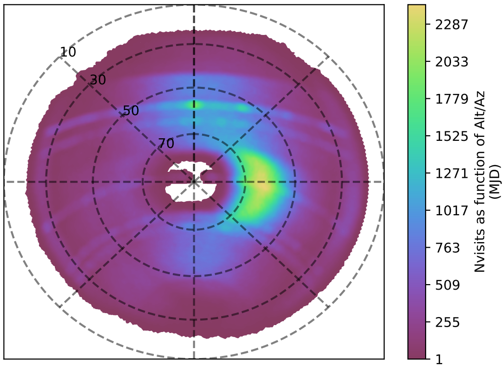
ddf_loaded_half_fl4_v3.4_10yrs i band: Nvisits as function of Alt/Az
