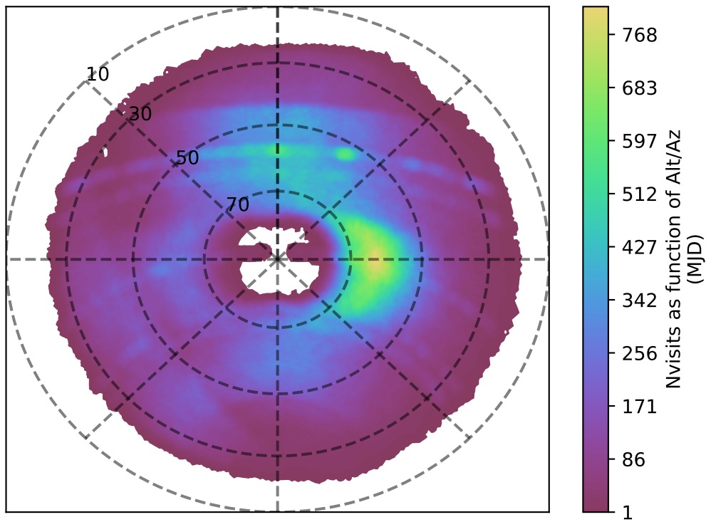
ddf_loaded_half_fl4_v3.4_10yrs g band: Nvisits as function of Alt/Az
