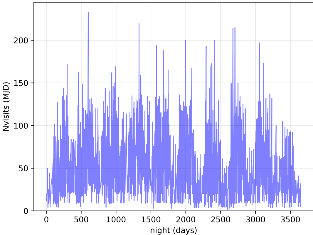
ddf_loaded_half_fl4_v3.4_10yrs DDF: Nvisits
