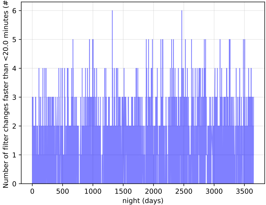
ddf_loaded_half_fl4_v3.4_10yrs Per Night: Number of filter changes faster than <20.0 minutes
