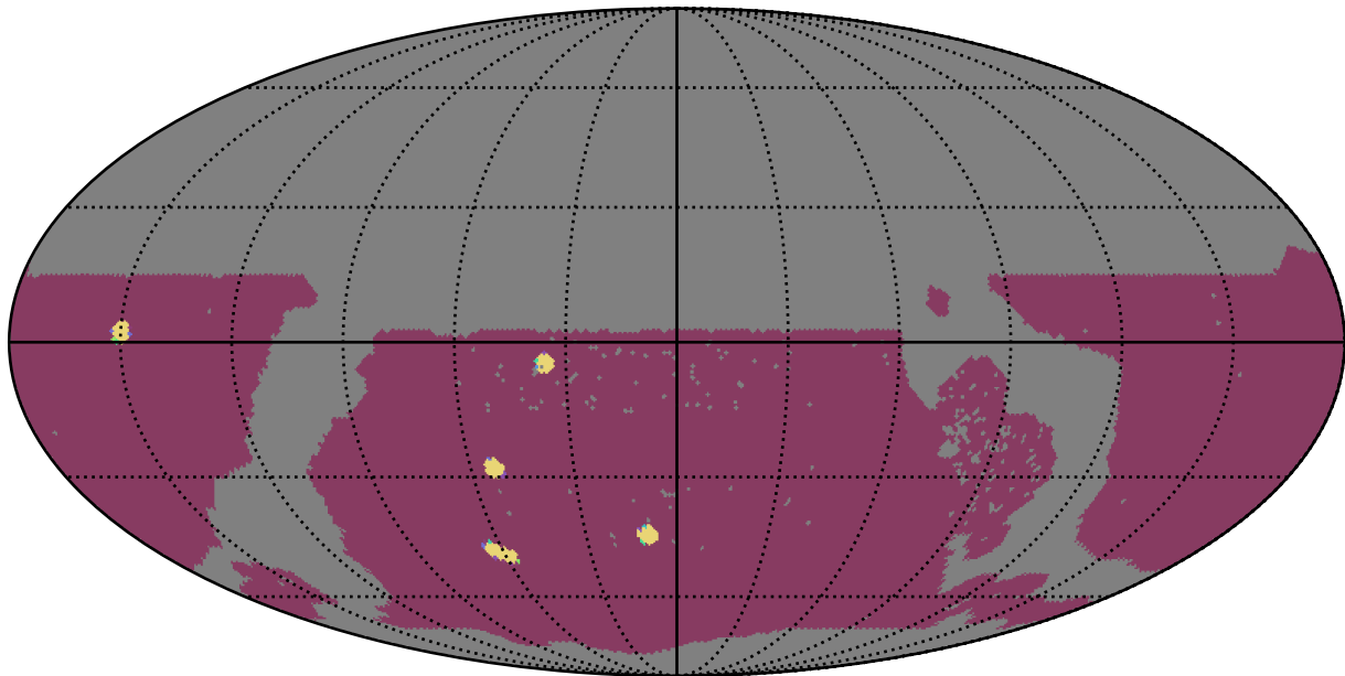
ddf_loaded_half_fl4_v3.4_10yrs WFD: NumberOfQuickRevisits
