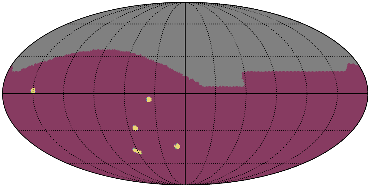
ddf_loaded_half_fl4_v3.4_10yrs All sky: NumberOfQuickRevisits
