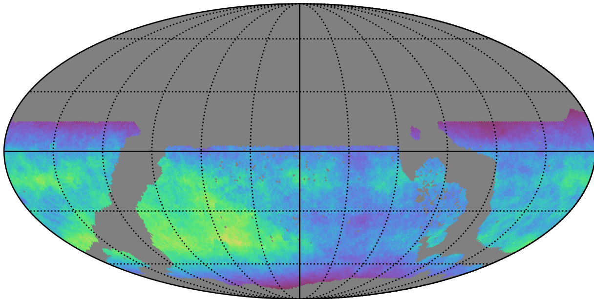
ddf_loaded_half_fl4_v3.4_10yrs WFD z band: Normalized Teff
