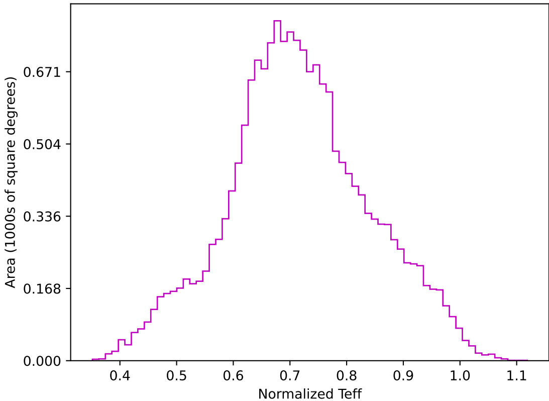
ddf_loaded_half_fl4_v3.4_10yrs WFD z band: Normalized Teff
