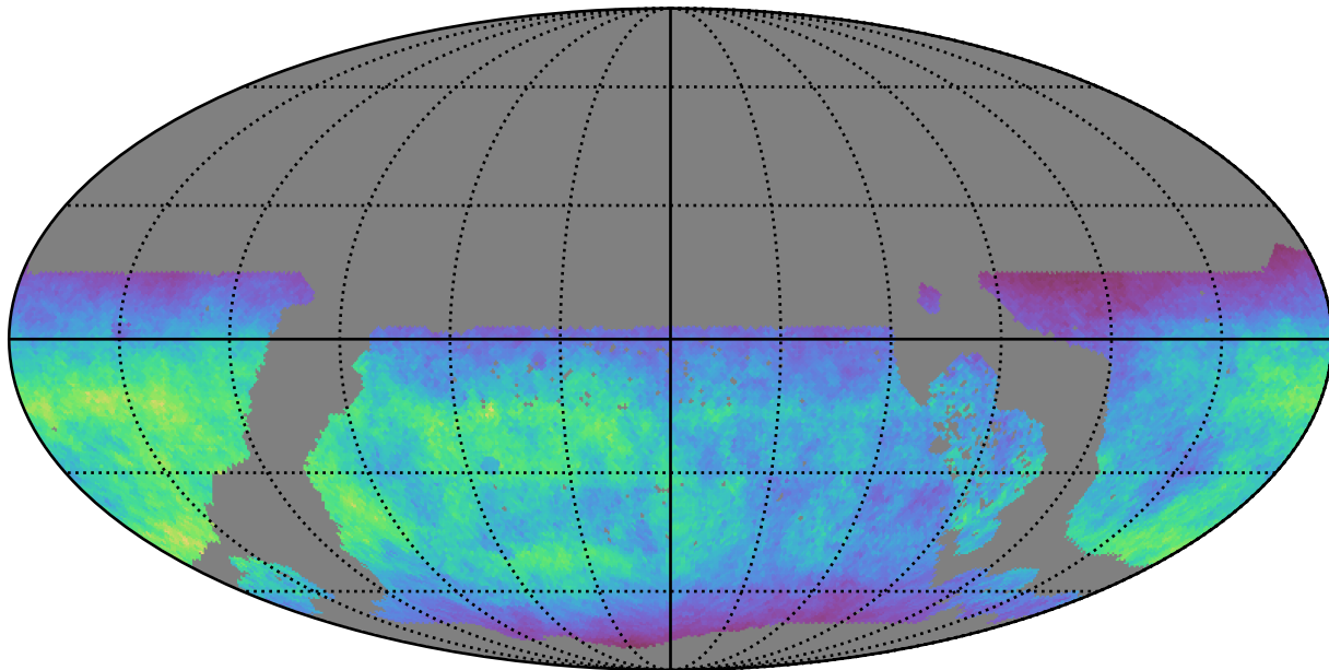
ddf_loaded_half_fl4_v3.4_10yrs WFD u band: Normalized Teff
