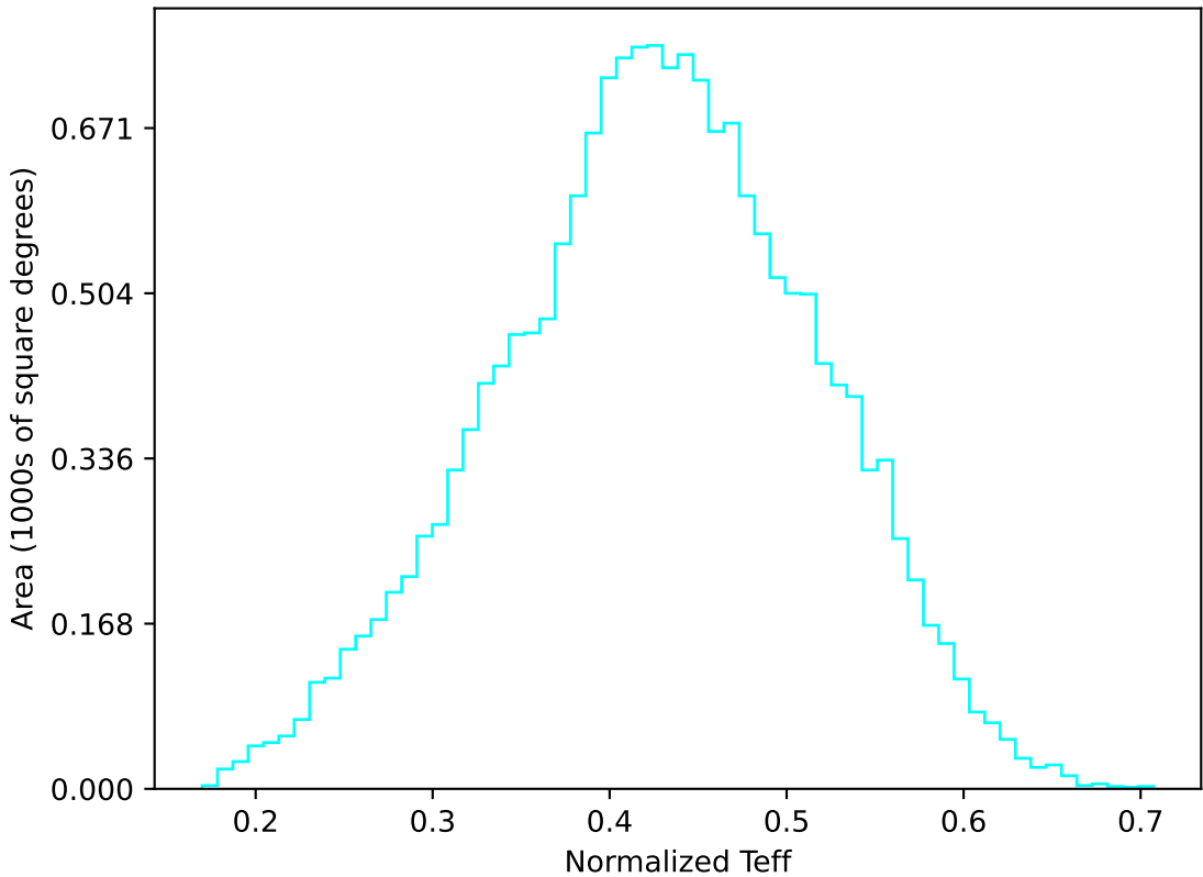
ddf_loaded_half_fl4_v3.4_10yrs WFD u band: Normalized Teff
