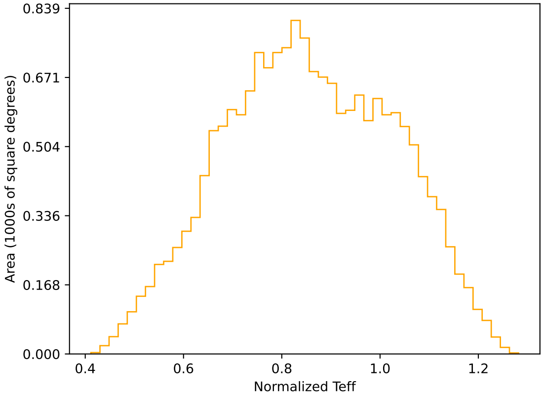
ddf_loaded_half_fl4_v3.4_10yrs WFD r band: Normalized Teff
