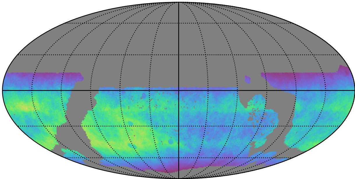
ddf_loaded_half_fl4_v3.4_10yrs WFD i band: Normalized Teff
