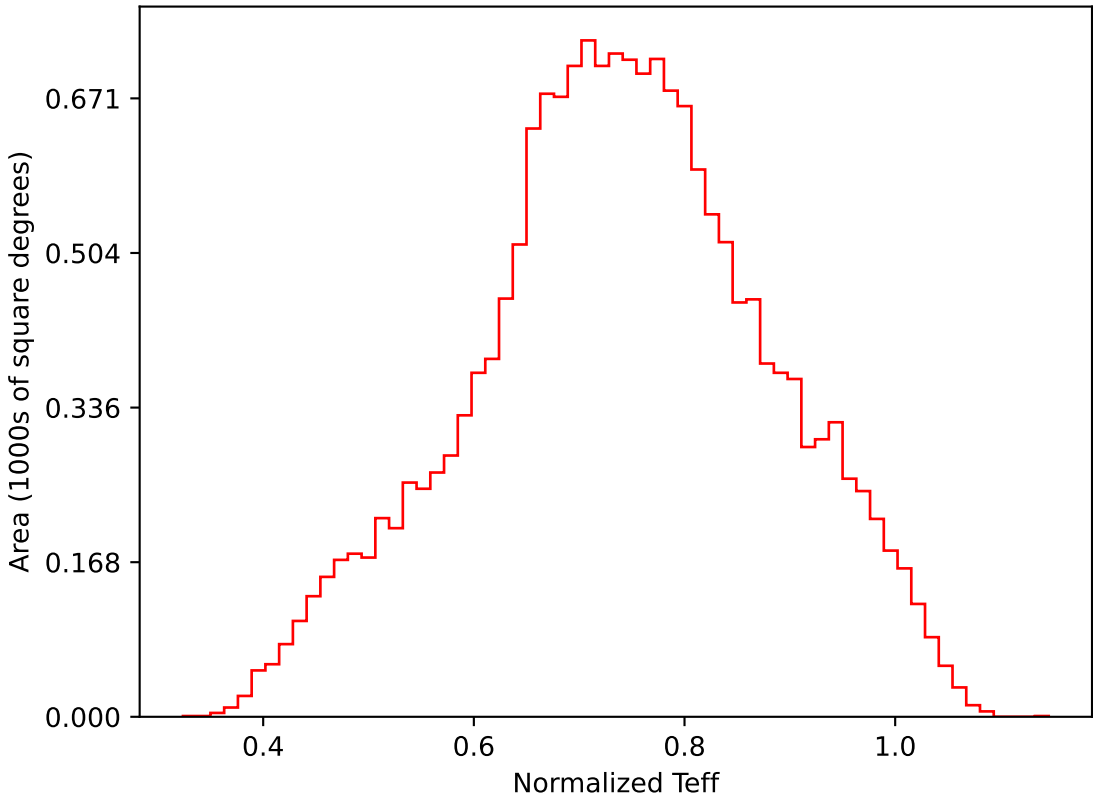
ddf_loaded_half_fl4_v3.4_10yrs WFD i band: Normalized Teff
